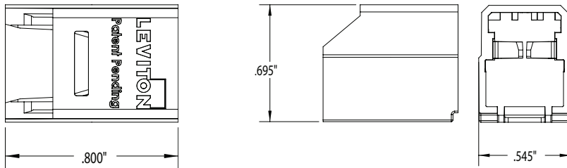
PORT BLOCKER
