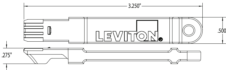
EXTRACTION TOOL
