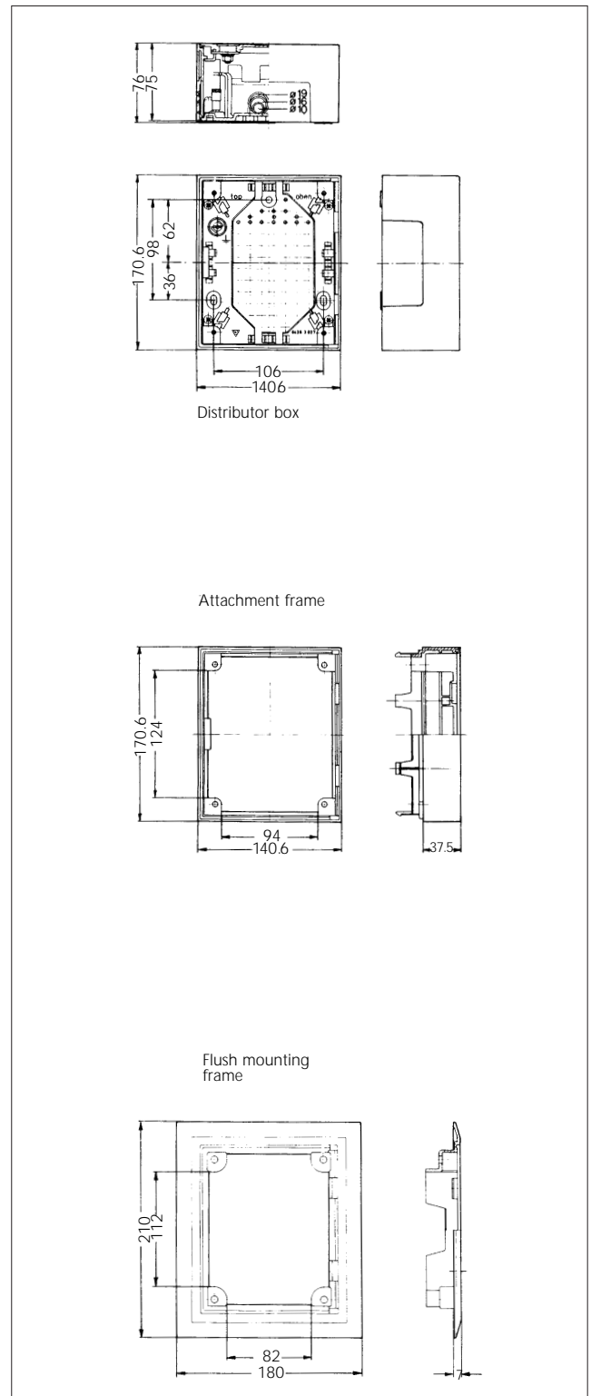
KRONECTION Box I for 30 pairs max.
