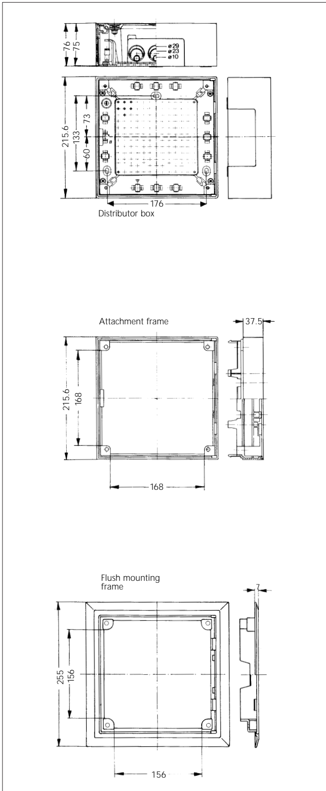
KRONECTION Box II for 50 pairs max.
