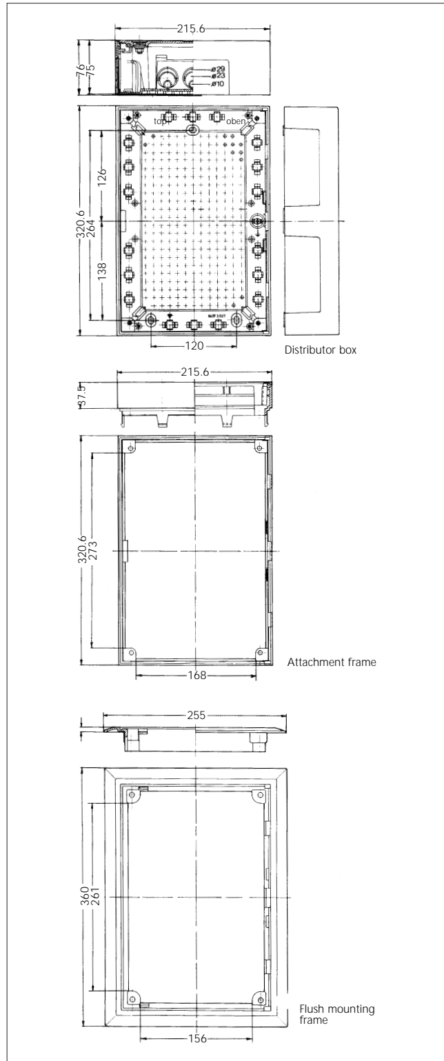
KRONECTION Box III for 100 pairs max.
